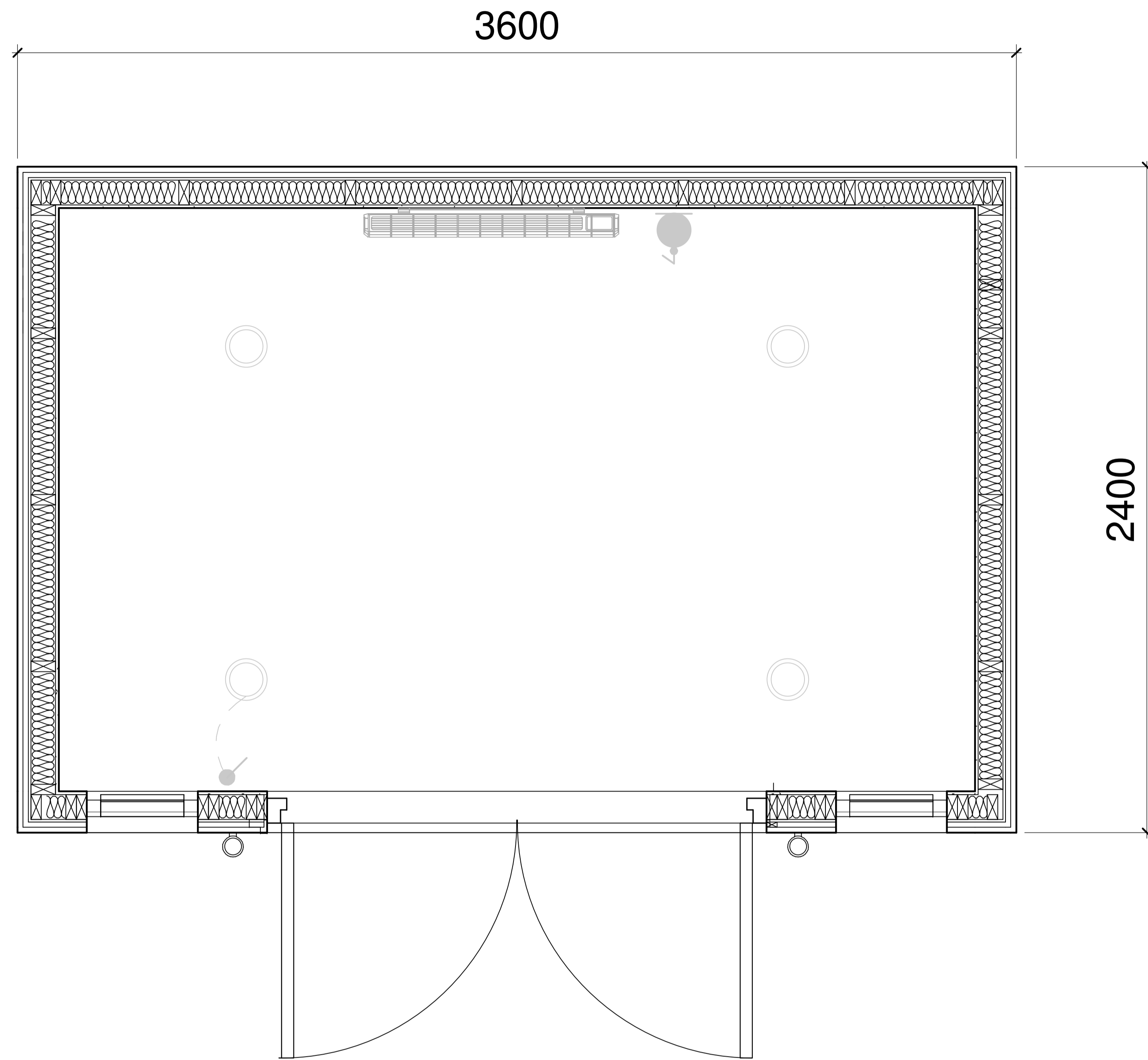
1 Proposed Layout 1 : 20
